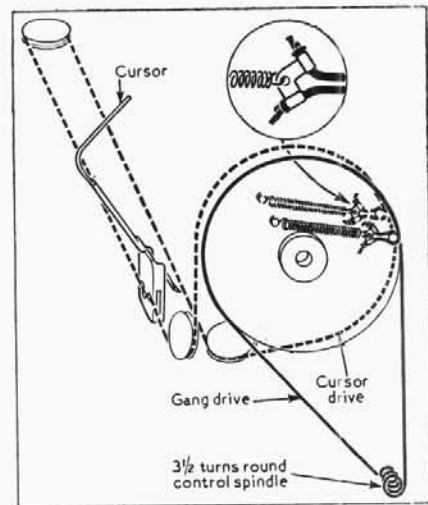
Sketch of the tuning drive system, which employs separate cords for gang drive and cursor drive. It is drawn as seen when viewed from the front right-hand corner of the chassis. Inset is shown the method of fixing the cord to the anchor plates.
